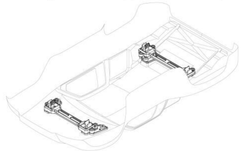
Completed Assembly (view from bottom)
