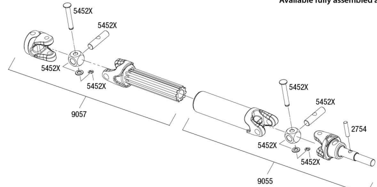
Rear Driveshaft Assembly Available fully assembled as part #9052
