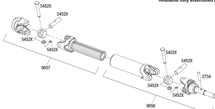
Front Driveshaft Assembly Available fully assembled as part #9051
